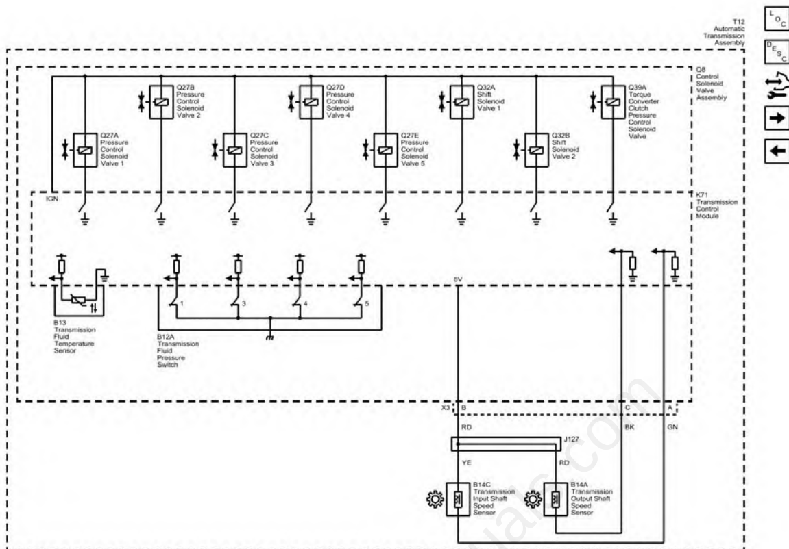
Fig. 2: Speed and Temperature Sensors, Pressure and Shift Controls
