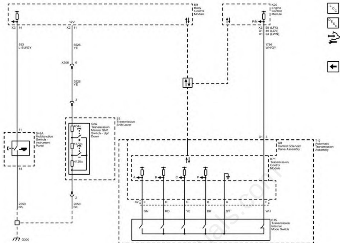
Fig. 3: Internal Mode and Tap Up/Tap Down Switches Courtesy of GENERAL MOTORS COMPANY
