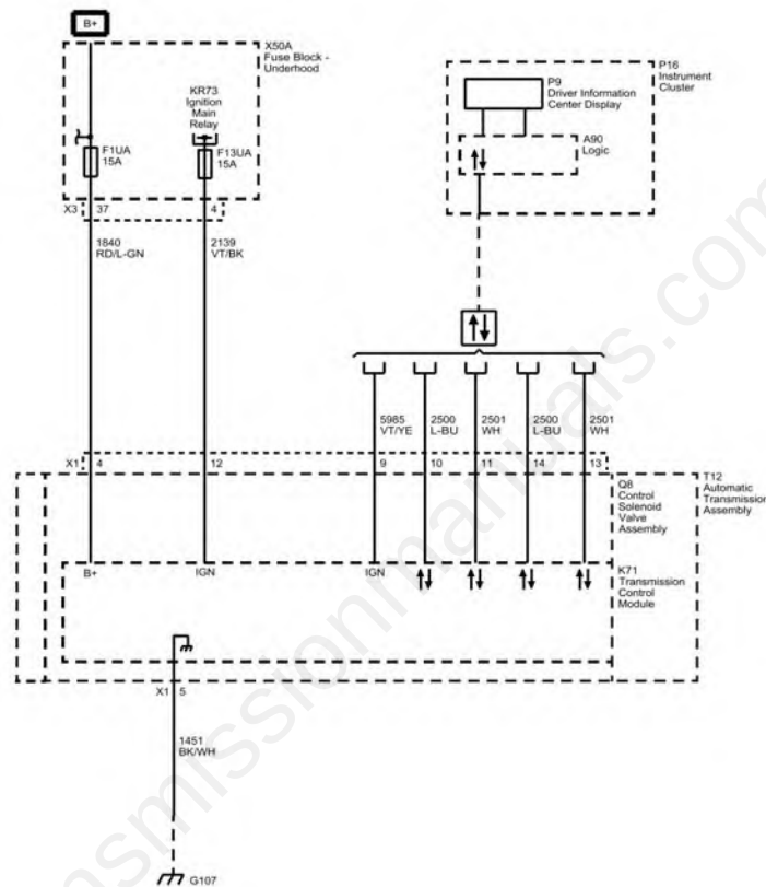
Fig. 1: Power, Ground, Data Communication, and MIL Courtesy of GENERAL MOTORS COMPANY
